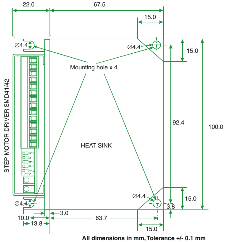
All dimensions in mm, Tolerance +/- 0.1 mm
