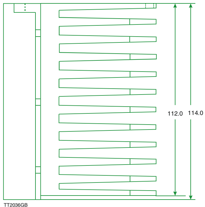
All dimensions in mm, Tolerance +/- 0.1 mm
